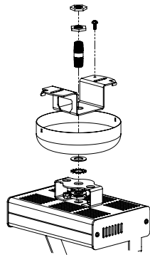
Typical Canopy Mount
