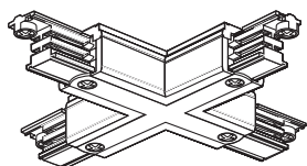
Feed-Able X Connector, 277V (ASL-HTEK38*)
