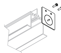
Recessed End Cap - Track jacket sold separately (ASL-FTP-241*)
