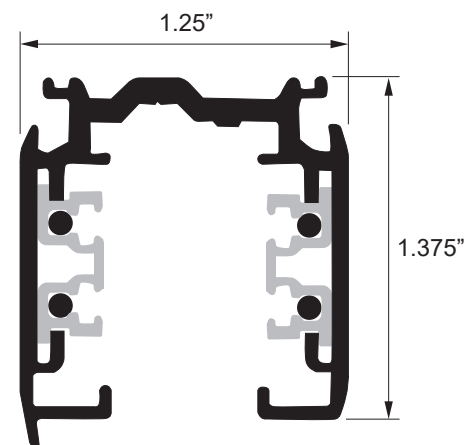
ASL-H2 Series Track
