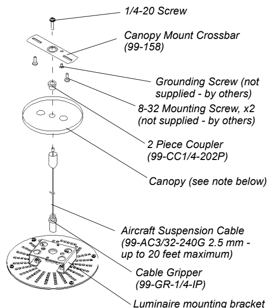
Figure 6: CDA70 Pendant Mount - Aircraft Cable
