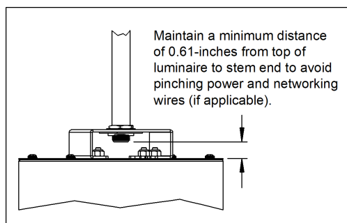
Figure 5: Stem Clearance
