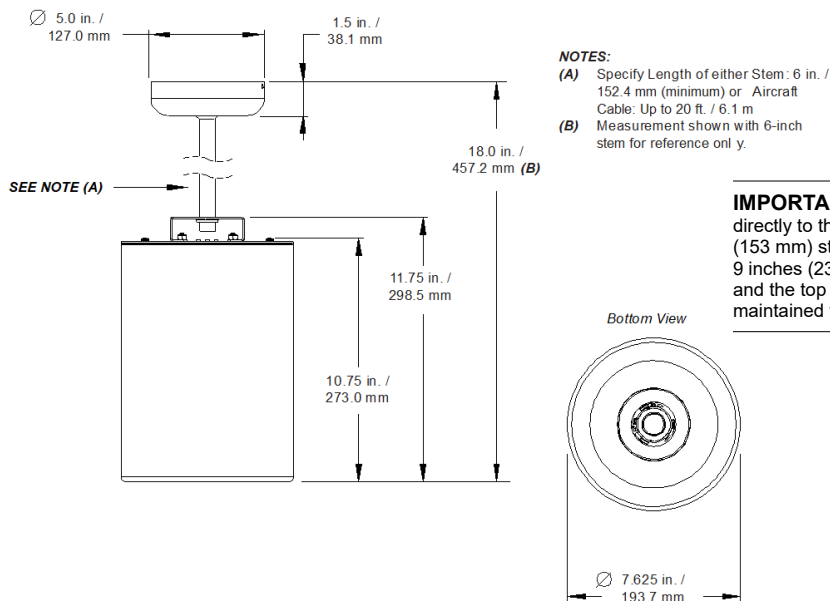
Figure 3: CDP70 Pendant Mount
