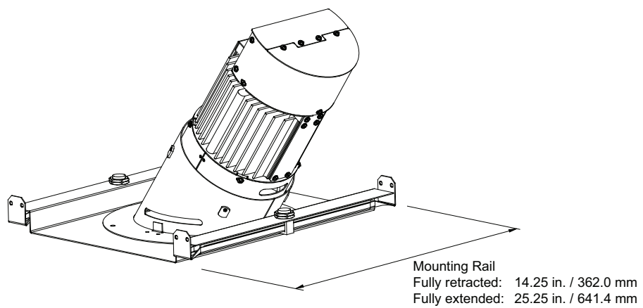
Figure 11: Sloped Ceiling Adapter Example
