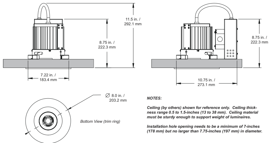
Figure 9: CDR70 Remodeler Mount
